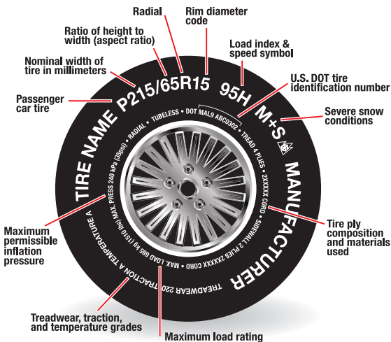
Figure 3: Typical Passenger Tire Markings
