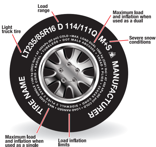
Figure 4: Typical Light Truck Tire Markings
